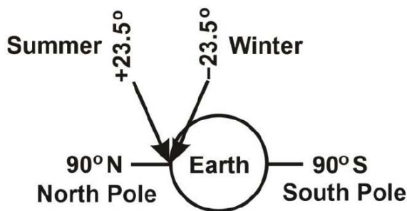
Figure 3: Sun angles for the Northern Hemisphere from summer to winter at the Equator and at the Poles.
