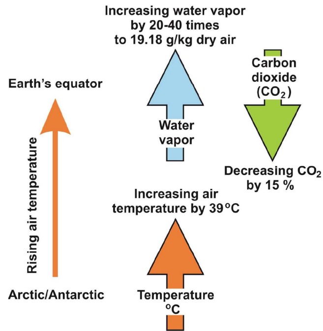
Figure 8: Actual relationship between temperature, water vapor and CO 2 when moving from the Poles to the Equator.
