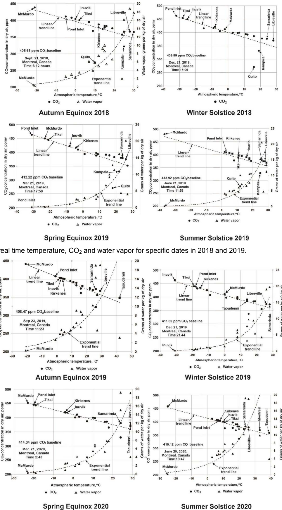
Figure 11: Plot of real time temperature, CO 2 and water vapor for specific dates in 2019 and 2020. Quito is replaced with Taoudenni, Mali, in the Sahara Desert.
